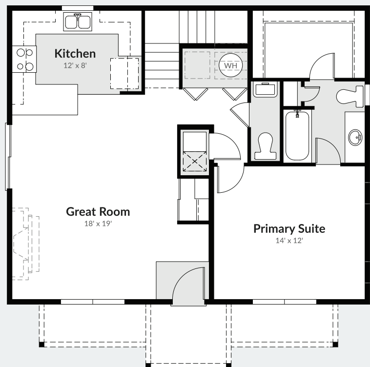
MAIN FLOOR
