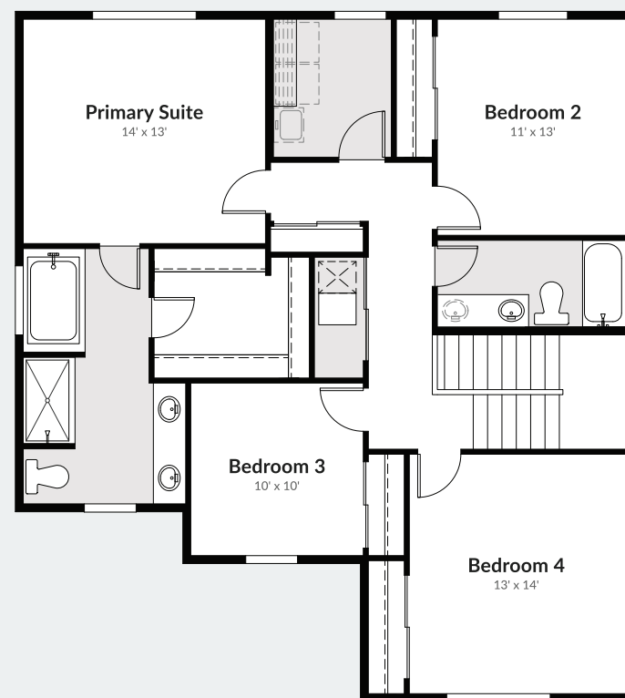
UPPER FLOOR
