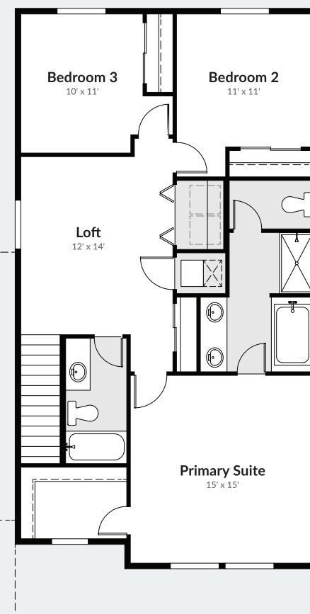
UPPER FLOOR
