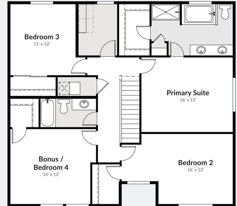
UPPER FLOOR
