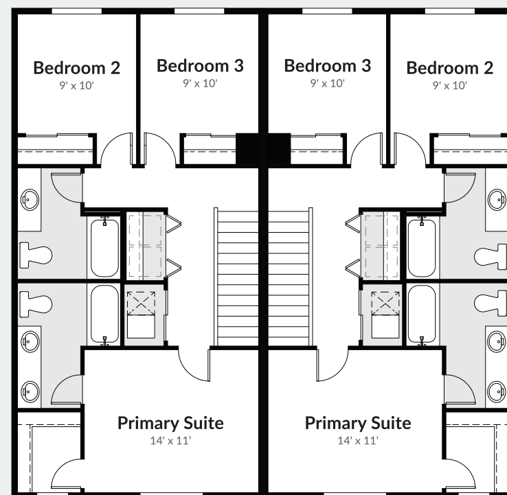
UPPER FLOOR
