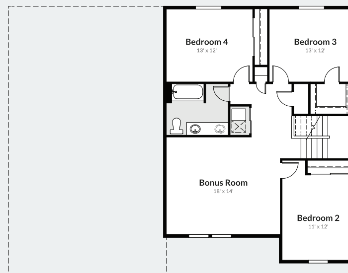
UPPER FLOOR
