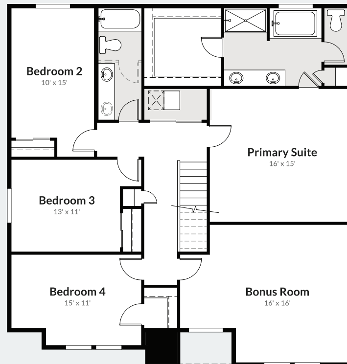
UPPER FLOOR
